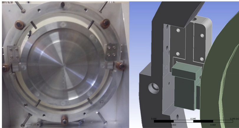
Figure 9. Prototype of the CP suspension and detail of the lateral clamps.
