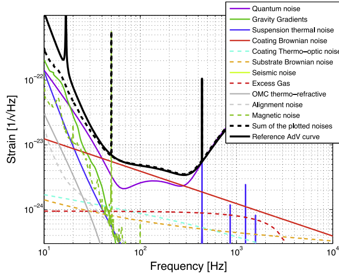
Figure 2. The AdV reference sensitivity (solid black) compared to an AdV noise budget (dashed black) using the new models for suspension thermal noise, gravity gradient noise and some modeled technical noises, computed in the configuration optimized for BNS detection with 125 W of input laser power. See section 2.1 for further details.
