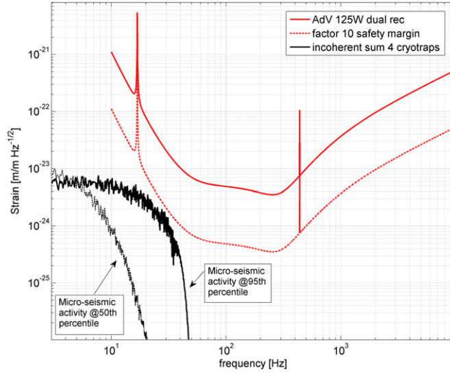
Figure 23. Projection of the displacement noise of the cryotrap baffles. The overall noise projection is estimated as the incoherent sum of the displacement noise coming from various baffle surfaces, multiplied by a factor of two to account for the four cryotrap of the arm cavities (incoherent sum). The solid line is for high microseismic activity (95th percentile upper limit), dashed line for usual microseismic activity (50th percentile upper limit).
