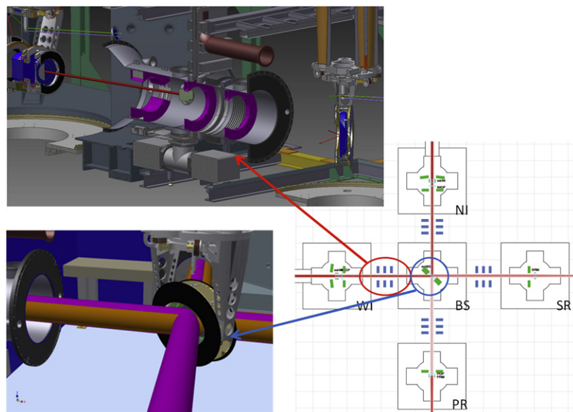
Figure 24. Schematics of the baffle positions inside the Central Area. Baffles connected to the vacuum links are depicted in blue, while the green baffles are suspended from the core optics-related SA. In the top-left panel, a 3D-section view of the baffles foreseen in the link WI-BS is shown, where clearance for the CO 2 laser for the TCS is made possible with a special baffle shape. The bottom-left panel shows a 3D rendering of the baffle integrated into the BS payload. Also depicted: beams impinging on the BS mirror travel clearly through the baffles.
