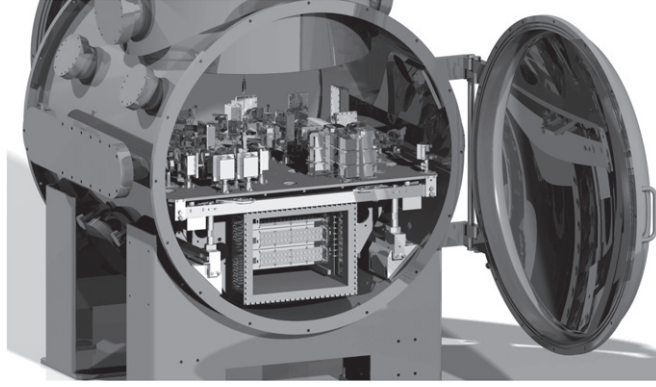
Figure 20. A 3D drawing of the new suspended bench inside its vacuum chamber.
