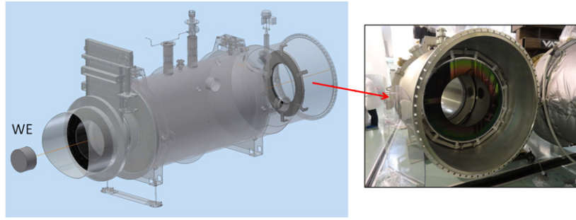
Figure 22. The large cryogenic traps separate the tanks housing the test masses from the long vacuum pipes of the arms. Inner structures need to be shielded from the test-mass view, so dedicated baffles are installed. The west end cryotrap was the first to be equipped with such baffles, shown in the right panel.
