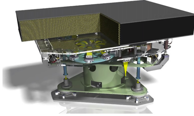
Figure 16. Impression of the external injection bench supported by the EIB-SAS. The EIB is a standard 2400 \times 1500 mm optical bench with a mass of 840 kg. The IP legs allow the intermediate platform ( spring-box ) to move horizontally. The spring-box hosts the three GAS springs, which allow the optical bench to move along vertical, pitch and roll DoF.
