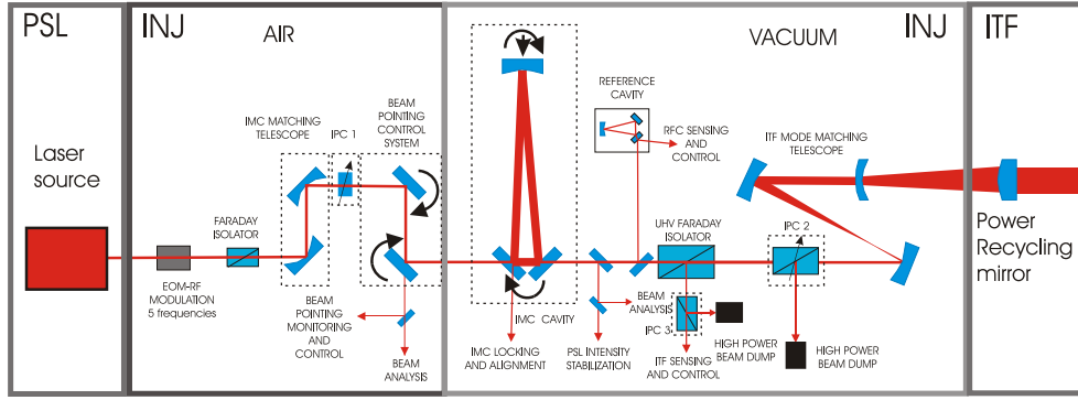
Figure 14. General input optics scheme.
