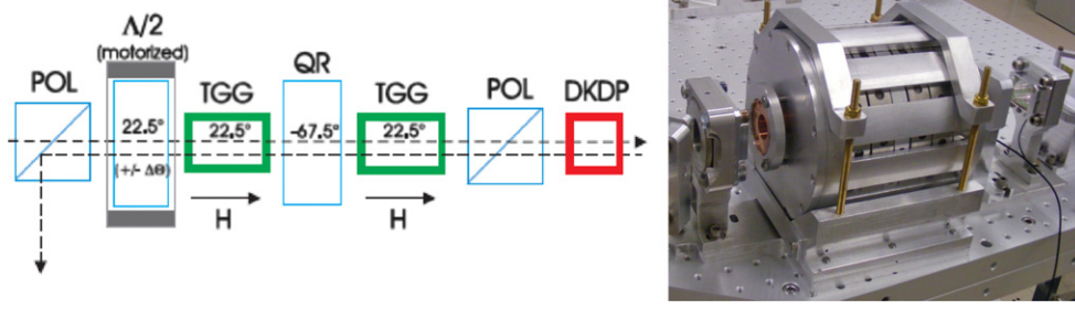
Figure 17. Left: a scheme of the HP-compatible Faraday isolator. Right: a view of the assembled device.
