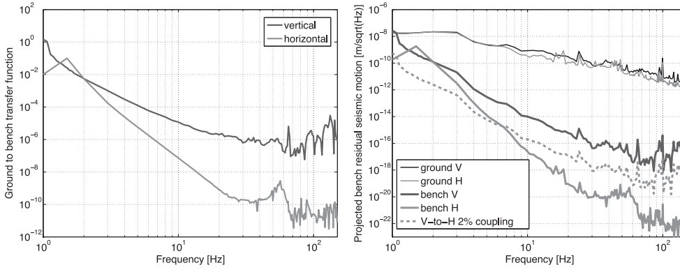
Figure 27. Left panel: MultiSAS measured vertical and horizontal transfer functions. A residual transmission around 10^{-6} is reached in the vertical. In the horizontal an attenuation limit around 10^{-9} is achieved above 20 Hz. The bump between 50 Hz and 60 Hz is due to the residual transmission around the GAS filter keystone modes. Right panel: estimated bench seismic motion in AdV. The residual horizontal displacement is expected to be dominated, above a few Hz, by the vertical-to-horizontal coupling, measured to be about 2%.
