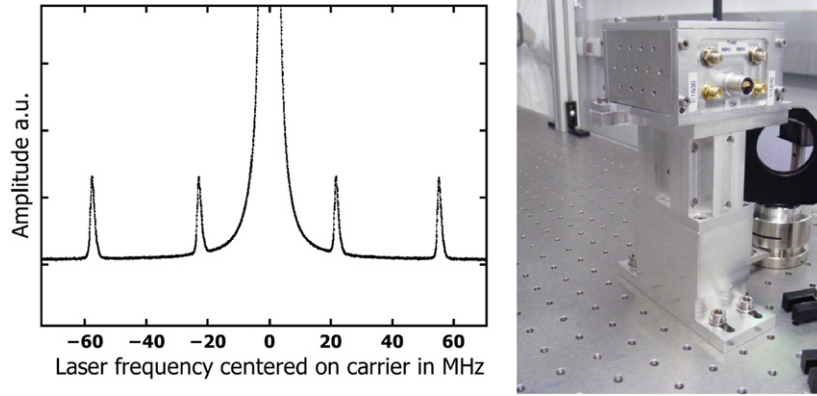
Figure 15. 22 MHz and 56 MHz sidebands, measured with a scanning FP cavity (left); AdV electro-optic modulator and the EIB.
