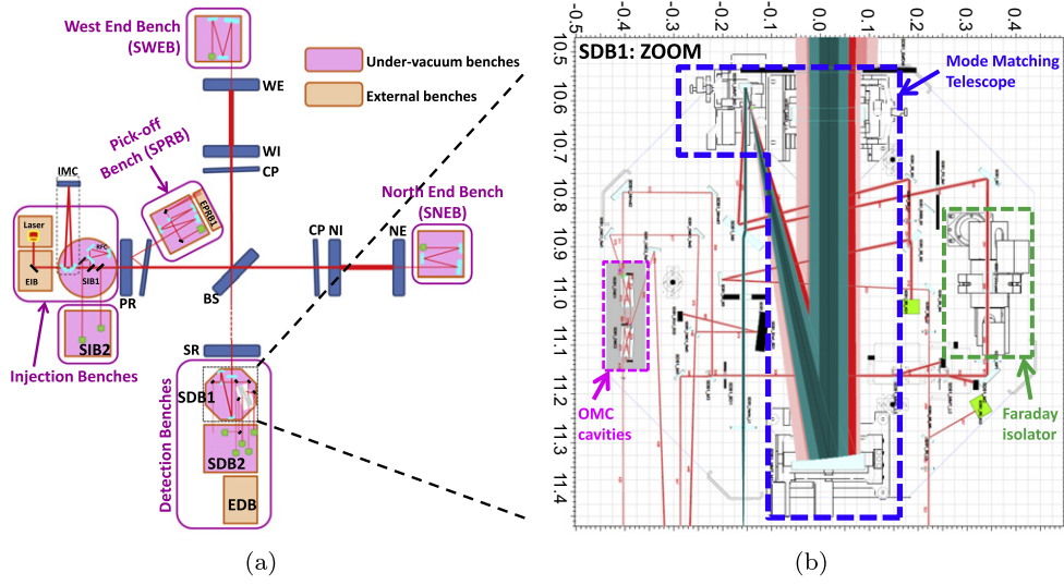
Figure 19. (a) A scheme of the optical benches foreseen for AdV. (b) The optical layout of the first suspended detection bench SDB1. YAG beams ( \lambda = 1064 nm) are displayed in red. A Hartmann beam ( \lambda = 800 nm) is displayed in green.
