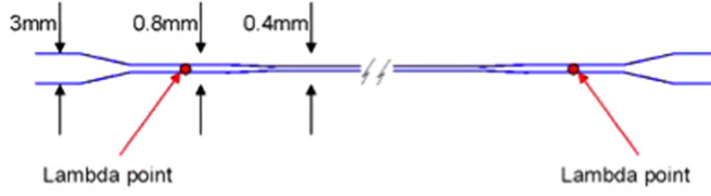
Figure 12. A sketch of the fused silica fiber shape in AdV.
