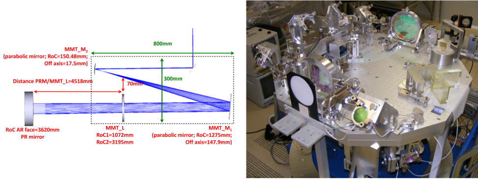
Figure 18. Catadioptric telescope of the SIB1 layout (left); MMT installed on SIB1 (right) in February 2014.
