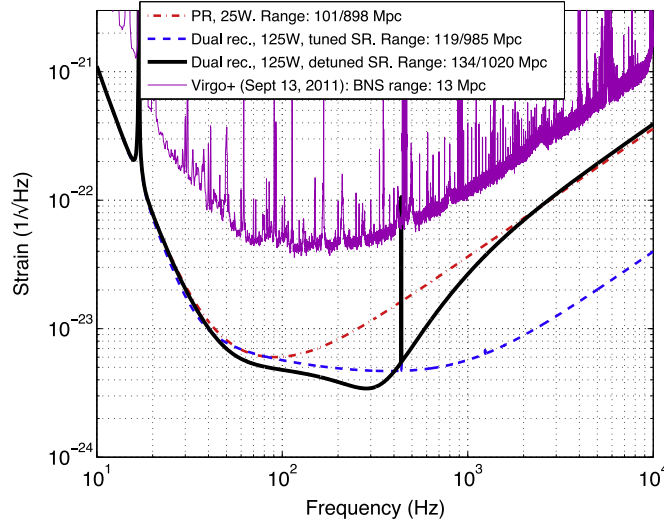
Figure 1. AdV sensitivity for the three benchmark configurations as defined in the TDR: early operation (dash-dotted line), 25 W input power, no SR; mid-term operation, wideband tuning (dashed line), 125 W input power, tuned SR; late operation, optimized for BNS (black solid line), 125 W input power, detuned SR (0.35 rad). In the legend, the inspiral ranges for BNS and BBH (each BH of 30 M_{\odot} ) in Mpc are reported. The best sensitivity obtained with Virgo+ is shown for comparison.
