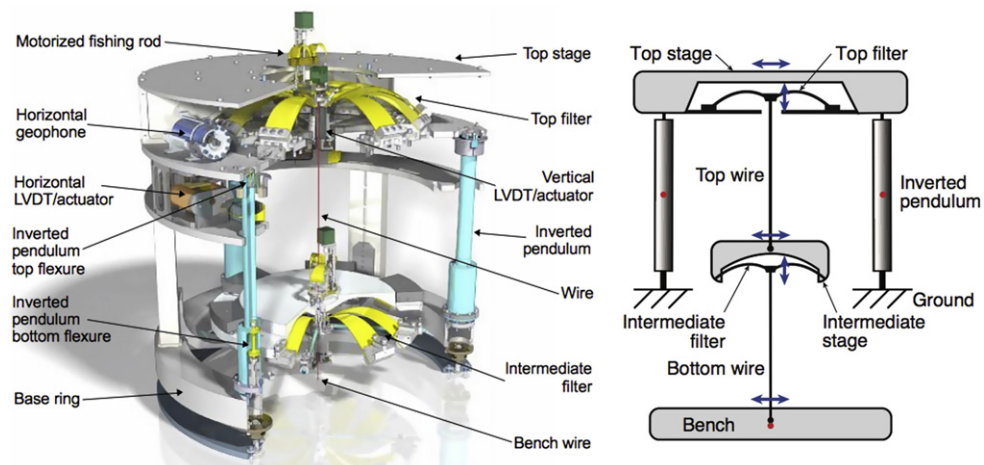
Figure 26. Left panel: MultiSAS overview. Right panel: MultiSAS conceptual design; two vertical (GAS springs) and three horizontal (IP and two simple pendulums) isolation stages are provided.
