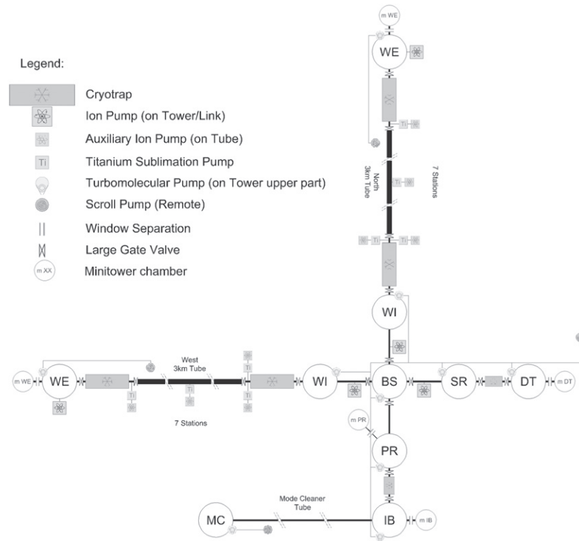
Figure 28. A schematic of the AdV pumping system.
