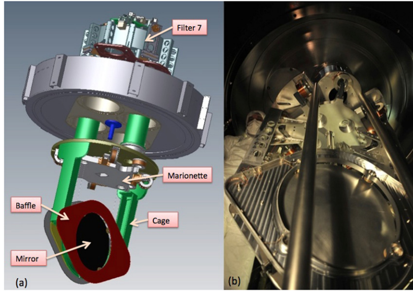
Figure 7. (a) Design of the new BS payload. (b) The prototype of the BS payload ready to be integrated with an SA for testing.
